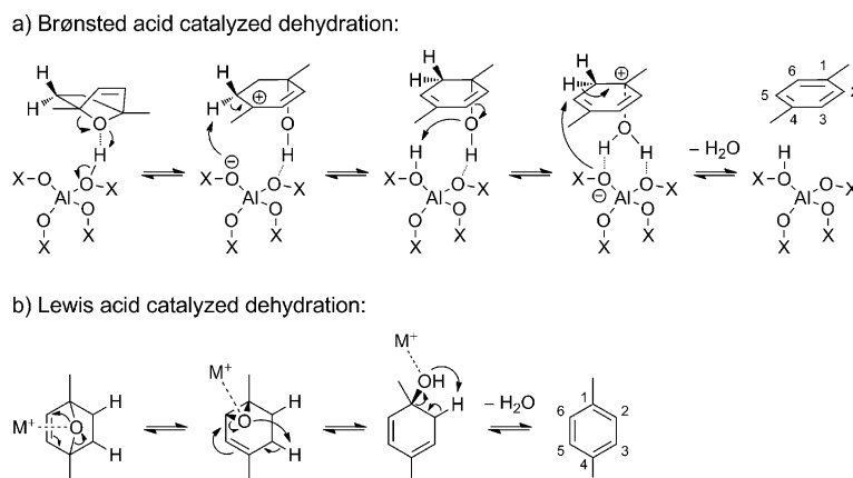
Scheme 4. Proposed mechanistic pathways for the a) Brønsted and b) Lewis acid catalyzed dehydration of 1,4-dimethyl-7-oxabicyclo[2.2.1]hept-2-ene to p -xylene. M = Li, Na, K, Rb, or Cs.
