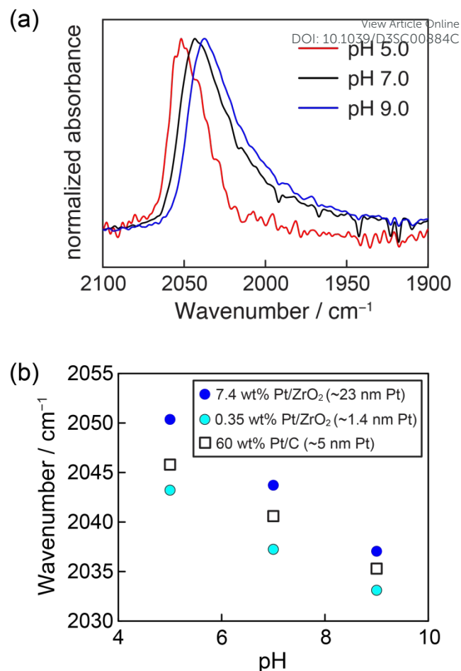
Figure 2. (a) pH-dependence of ATR-IR spectra at saturation of atop CO adsorbed on 7.4 wt% Pt/ZrO 2 immersed in aqueous buffered electrolyte solutions. (b) pH-dependence of the peak maximum for atop-bound CO adsorbed on 7.4 wt% Pt/ZrO 2 (~23 nm Pt nanoparticles), 0.35 wt% Pt/ZrO 2 (~1.4 nm Pt nanoparticles), and 60 wt% Pt/C (~5 nm Pt nanoparticles). The data for 60 wt% Pt/C are reproduced here from ref. 14. Conditions: 7 kPa CO, 94 kPa H 2 , electrolyte = 0.5 M NaClO 4 in Britton-Robinson universal buffer (0.04 M acetic acid, 0.04 M phosphoric acid, 0.04 M boric acid in water); pH adjusted with NaOH; performed at room temperature (294 ± 1 K).
