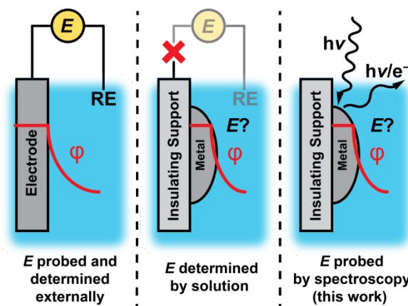
Figure 1. Different approaches for controlling and measuring solid-liquid interfacial polarization and potential of conductive and insulating materials. Traditionally, (a) wired experiments allow for the direct measurement of interfacial potential, while on (b) insulating-support-based metals, potentials are not as easy to determine. We report a method based on (c) a combination of X-ray photoelectron and vibrational spectroscopies to directly measure the electrochemical potential of metals supported on insulating materials.
