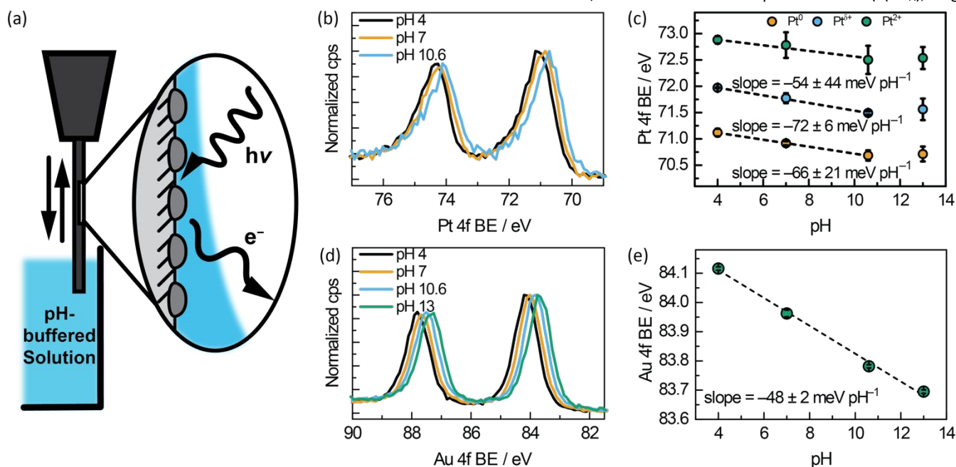
Figure 3. (a) Schematic of our AP-XPS measurement for \text{ZrO}_2 -supported metal nanoparticles after dip and pull in aqueous buffered electrolyte solutions of varying pH (ranging from pH 4 – 13) under constant \text{H}_2 pressure of \sim 0.5 kPa. (b) Pt 4f spectra, corrected based on the Na 1s spectra, of \text{ZrO}_2 -supported Pt nanoparticles ( \sim 8 nm) immersed in solutions of varying pH. (c) pH-dependence of Pt 4f binding energies using a three-component fit for Pt. (d) Au 4f spectra, corrected based on the Na 1s spectra, of \text{ZrO}_2 -supported Au nanoparticles ( \sim 8 nm) immersed in solutions of varying pH. (e) pH-dependence of Au 4f binding energies using a one-component fit for Au. The fitting protocol and error analysis are described in the SI.
