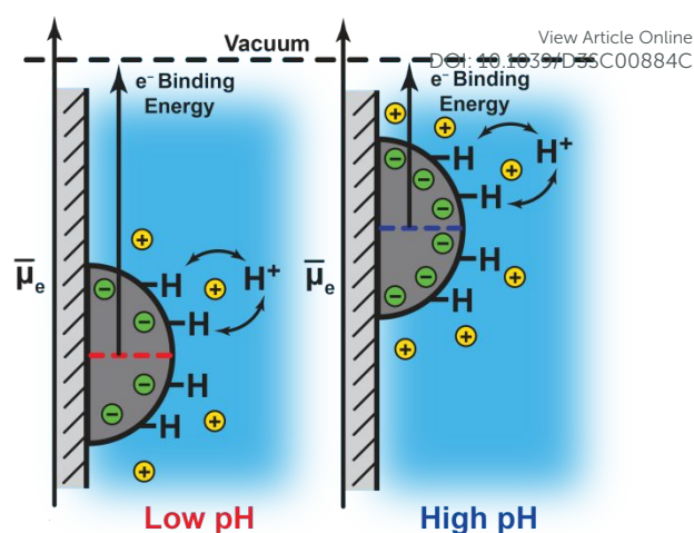
Figure 4. pH-dependent surface charging of insulator-supported metal particles and the attendant shift in the electrochemical potential of electrons, \bar{\mu}_e , which equals the Fermi level of the metal particles.
