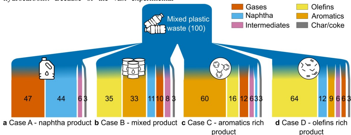
Fig. 1. Overview of product mass distributions across the four scenarios considered in this study. (a) Case A – naphtha product. Here, the hot effluent vapor stream from the pyrolysis section is quenched to yield a naphtha-rich liquid stream comprising gasoline-range, diesel-range, and high-boiling-point hydrocarbons (>370°C). (b) Case B – mixed product. The vapor stream is quenched to separate an olefins-rich gaseous stream (total olefins yield = 35 wt%) and an aromatics-rich liquid stream (total aromatics yield = 33 wt%). (c) Case C – aromatics-rich product. The process design highlights the maximum production of aromatic chemicals of up to 60 wt% (trade-offs with olefins yield) using a catalyst-to-feed (C/F) ratio of 4. (d) Case D – olefins-rich product. The process diagram highlights the greater yield of olefins. The process intermediates including char and heavies are utilized to generate heat for the pyrolysis reactor operation in all the cases.
