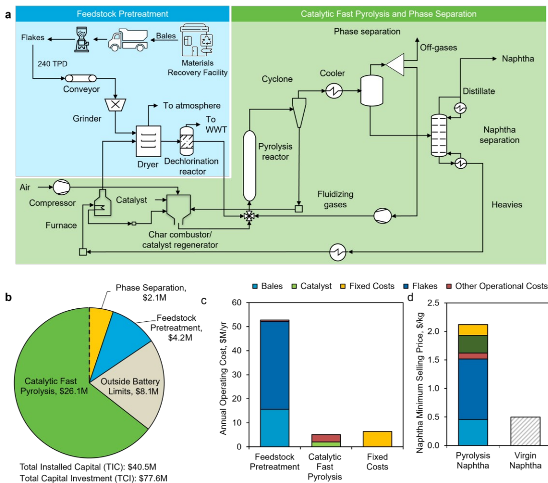
Fig. 2. TEA Results for Case A – naphtha product. (a) Process flow diagram of Case A. The pre-processed feedstock is catalytically pyrolyzed in an in situ fast pyrolysis reactor to produce a 50 wt% liquid naphtha stream that primarily contains gasoline (44 wt%) and diesel fractions. The aromatic content of the gasoline fraction is 76 wt%. (b) Capital cost breakdown by area for each process section, with a total installed capital (TIC) of $40.5 million and total capital investment (TCI) of $77.6 million. This includes $8.1M contribution assumed from the outside battery limits (OSBL) investment (OSBL is 25% of inside battery limits, ISBL), which consists of additional capital expenditure including piping and instrumentation required to integrate the over-the-fence utilities into the plant. (c) Annual operating expense by process section. Fixed costs include fixed variable expenses toward labor, maintenance, and property and insurance taxes. Other operational costs include utilities like process steam, cooling water, and natural gas for the operation of the facility. (d) MSP breakdown of the naphtha case. The MSP of naphtha from pyrolysis of mixed plastic waste is $2.18/kg, which is approximately 4-fold higher than that of fossil-derived naphtha ($0.50/kg).
