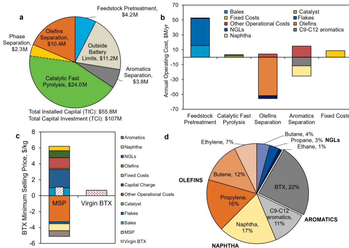
Fig. 4. TEA results of Case B – mixed product. (a) Capital cost breakdown by area for each process section, with total installed capital (TIC) of $55.8 million and total capital investment of $107 million. (b) Annual operating expenses for the base case, disaggregated by process step (total = $84 million/yr). The highest contribution is from feedstock costs. Fixed costs include labor and overhead. Note that BTX is not considered a co-product in estimating the annual operating expenses. (c) The minimum selling price (MSP) breakdown of BTX aromatics relative to virgin BTX manufacturing. (d) The contribution of co-products towards the MSP. Aromatics streams comprise BTX and C 9 –C 12 aromatics. Natural gas liquids (NGLs) consist of ethane, propane, and butane. All data shown in Fig. 4 are included in Tables S4–S6 for Fig. 4a, Table S7–S12 for Fig. 4b, and Tables S13–S14 for Fig. 4c.
