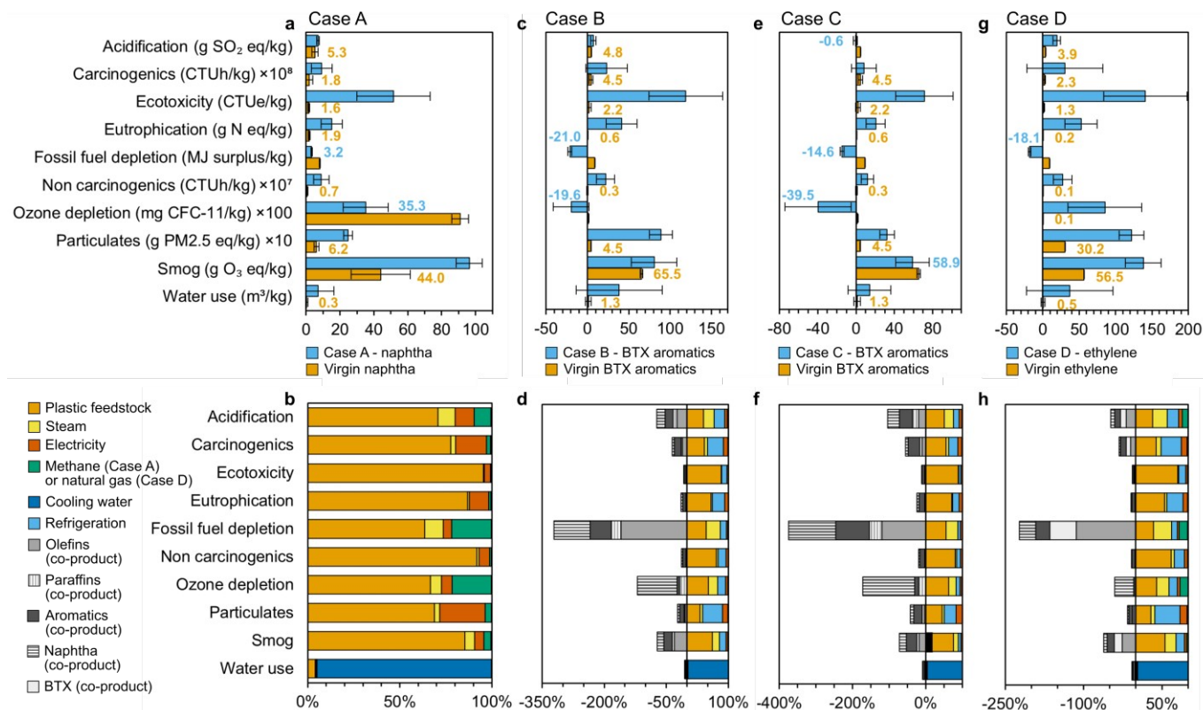
Fig. 7. Life cycle assessment for pyrolysis of mixed plastic waste to naphtha, BTX aromatic mixtures and ethylene under different process scenarios. (a) Comparison of the Case A – naphtha product to virgin naphtha, (b) Contributions of various process components to the overall environmental impacts of the Case A. (c) Comparison of the Case B – mixed product (where principal product is BTX aromatic hydrocarbons) to virgin BTX mixture, (d) Contributions of various process components to the overall environmental impacts of the Case B. (e) Comparison of the Case C – BTX aromatics rich product to virgin BTX aromatic mixture, (f) Contributions of various process components to the overall environmental impacts of the Case C, (g) Comparison of the Case D – ethylene monomer product to virgin ethylene, (h) Contributions of various process components to the overall environmental impacts of the Case D. Aromatic co-products include C 9 –C 12 aromatics, paraffin co-products include ethane, propane, and butane, and olefin co-products include ethylene, propylene, and butene. Components with contributions less than 1% (catalyst, process water, dimethylformamide (DMF) solvent, infrastructure, and wastewater treatment) are not included in the figure. Calculations were conducted with TRACI 2.1 US 2008 and AWARE methods, SimaPro software, and ecoinvent 3.3 background data. All data shown in Fig. 7a-h are included in numerical form in Tables S23-S26 .
