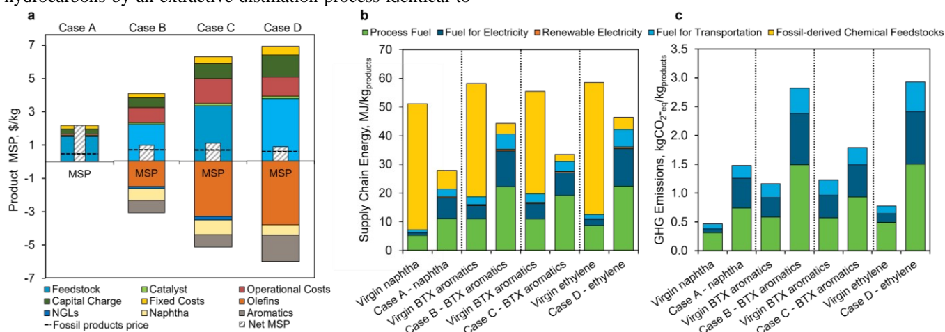
Fig. 6. Comparative summary of the economic and environmental analysis of the different pyrolysis scenarios proposed in this study. (a) Economic summary: Case A shows the MSP breakdown of naphtha product as a function of process variables, Case B shows the MSP breakdown for BTX aromatic hydrocarbons. The MSP of $1.07/kg is 1.6 times higher than virgin BTX aromatic hydrocarbons ($0.68/kg). Case C – aromatics-rich product has BTX aromatic hydrocarbons as the main product and is estimated at an MSP of $0.95/kg. Finally, Case D – olefins-rich product with ethylene as the main product is estimated at an MSP of $0.85/kg, which is 1.4 times that of virgin ethylene ($0.61/kg). Note that dotted lines show the price of fossil-derived products for the respective cases. (b) Supply chain energy and (c) GHG emissions of the four cases relative to virgin manufacturing. Fig. S9 illustrates a comparison of GHG emissions calculated by MFI versus LCA. Fig. S10 shows the system boundaries for the MFI analysis. All supply chain energy and GHG emissions data are in Tables S19–S22 .
